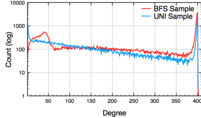
Fig. 5. Degree distribution
