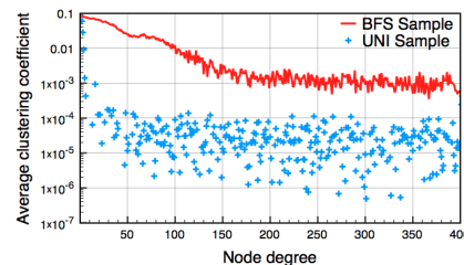
Fig. 8. Clustering coefficient
