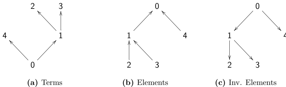
Figure 4. Isomorphic Graphs
