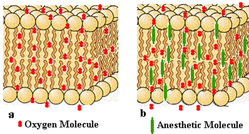
Figure 4. Illustration of anesthetic action. a shows the normal diffusion of O_2 without anesthetics dissolved into neural membranes. b shows anesthetic perturbations of O_2 pathways and neural membranes themselves.
