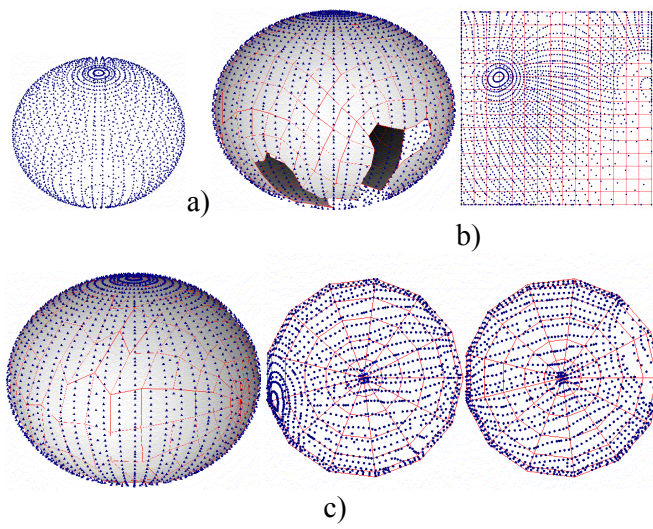
Fig. 14: Distribution of points on the sphere
