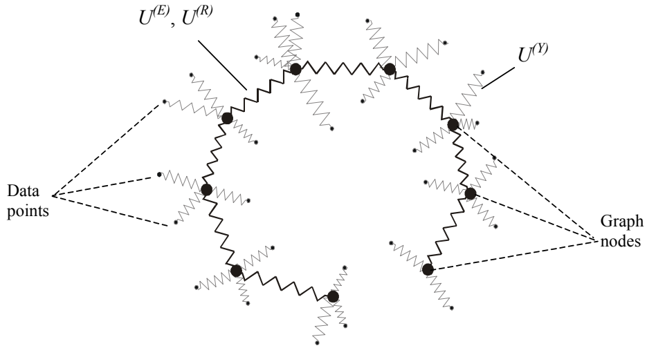
Fig. 3: Energy of elastic net
