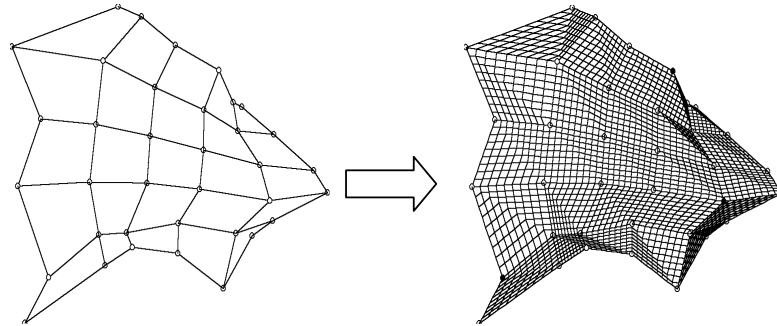
Fig. 6: Piecewise linear manifold
