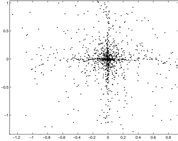
Fig. 4. Separation performed by the MLP-based network.
