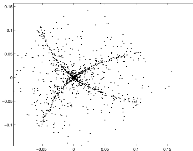
Fig. 3. Mixture of supergaussian sources.
