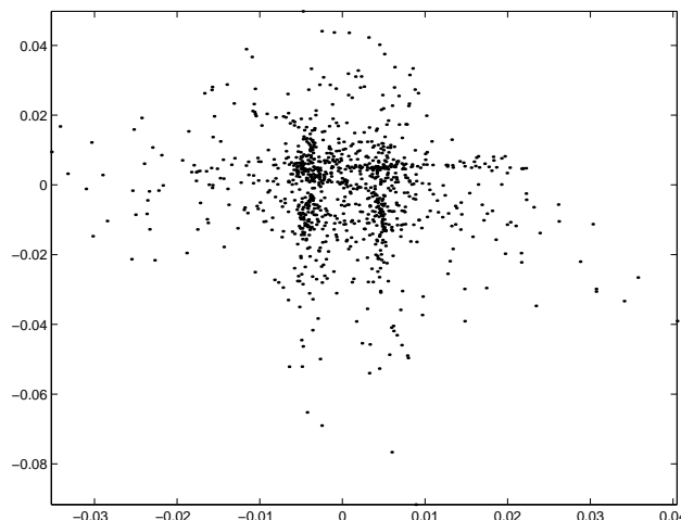
Fig. 9. ICA result obtained with the RBF-based network without regularization, in the case of the mixture of two supergaussians.
