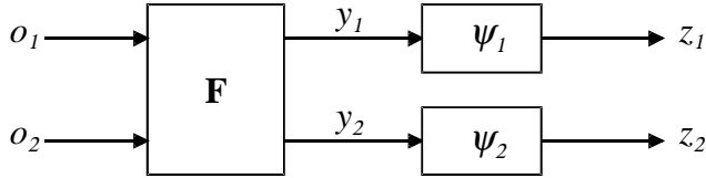
Fig. 1. Structure of the ICA systems studied in this paper. In the INFOMAX method the nonlinearities \psi_i are fixed a-priori. In the MISEP method they are adaptive, being implemented by MLPs.
