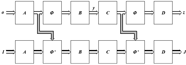
Fig. 2. Network for computing the Jacobian.
